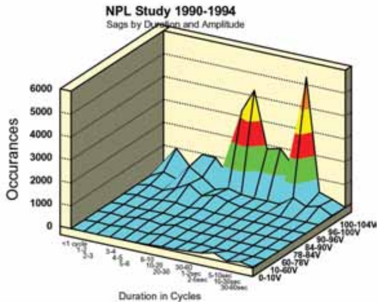
Figure 1. Number of Occurances of Magnitude versus Duration of Sags from NPL Survey
