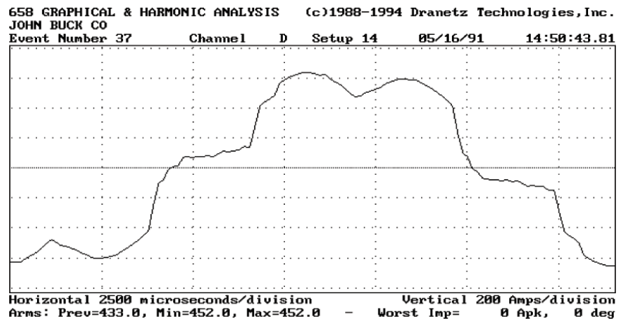
Figure 3. Current Waveform from 6-pole converter.
