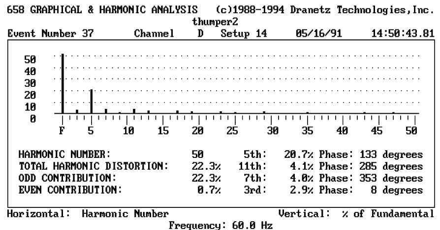
Figure 4. Harmonic Spectrum from Figure 3.
