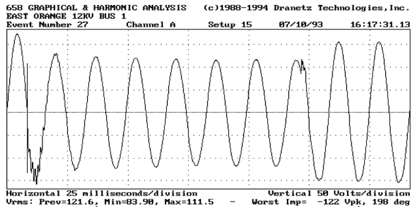
Figure 5. Voltage Sag From Distribution Level Fault
