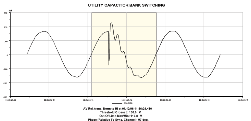
Figure 6. Power Factor Correction Capacitor Switching Transient.
