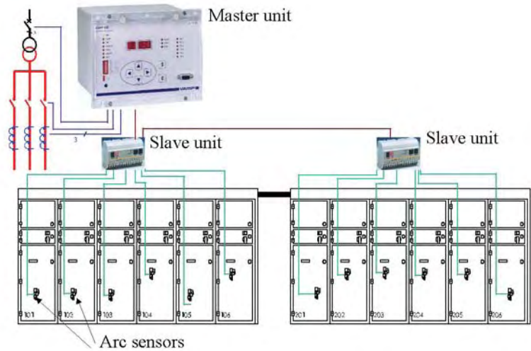
Figure 4: Structure of an arc protection system.
