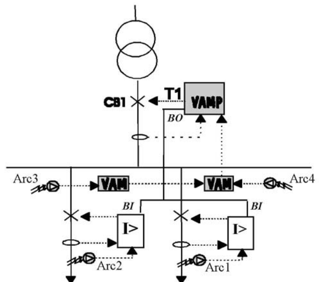
Figure 7: Overcurrent relays with arc sensor option and specialised arc protection system (VAMP and VAM). Information about activation of arc sensors Arc3 and Arc4 is also brought to the overcurrent relays via the binary inputs (BI).
